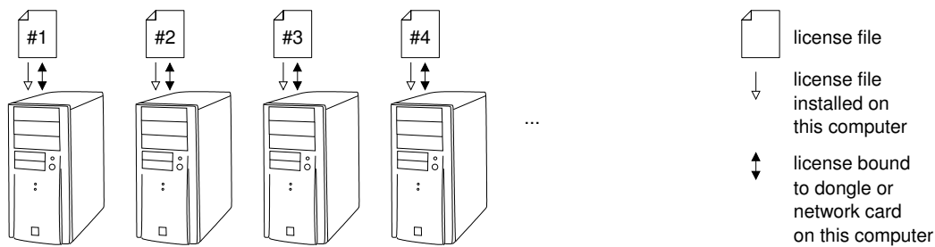
Figure 3.1: Individual node-locked licenses.
